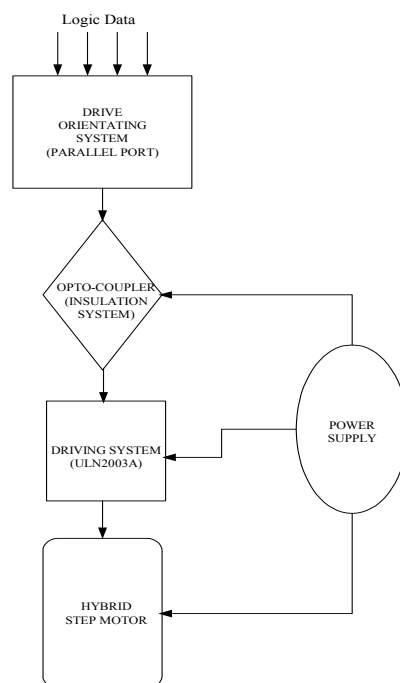
Fig. 1. The interaction between Visual package and hybrid step motor via PC's parallel port and the process of data transmitting
