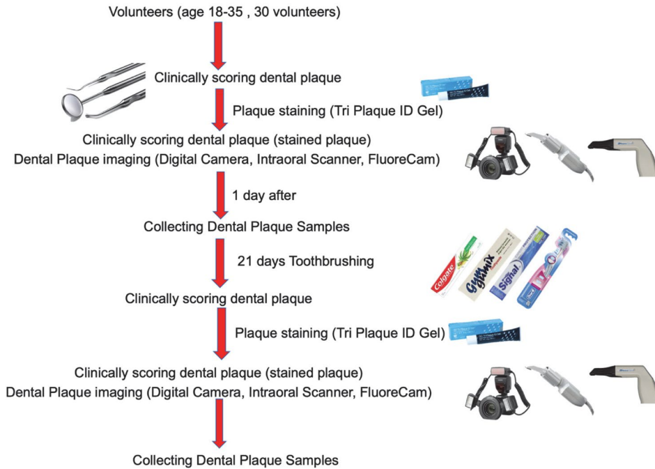
Fig. 1. Study workflow.
