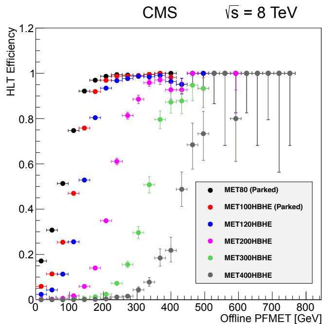
Figure 44. The HLT efficiencies as a function of the offline PF E_T^{\text{miss}} for different E_T^{\text{miss}} thresholds ( E_T^{\text{miss}} = 80 – 400 GeV).
