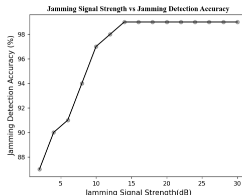
FIGURE 15: Jamming detection accuracy vs jamming signal strength
