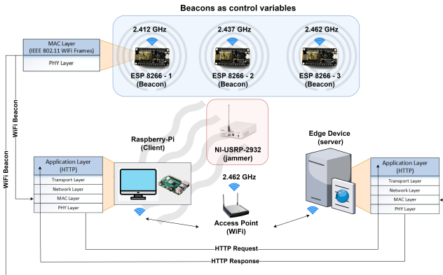
FIGURE 3: Experimental Setup
