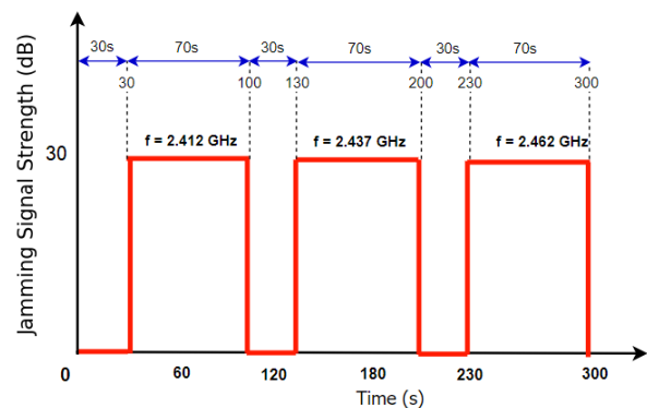
FIGURE 4: Jamming signal pattern for Experiment-1
