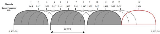
FIGURE 1: Channels in 2.4 GHz Wlan band
