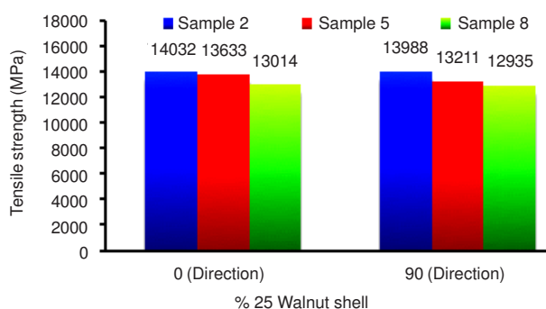
Fig. 5. Resistance results of composite materials containing 25 % walnut shell
