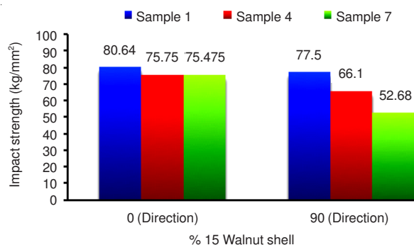
Fig. 10. Impact strength results of composite materials containing 15 % walnut shell
