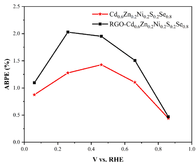
Fig. 12. ABPE values for \text{Cd}_{0.6}\text{Zn}_{0.2}\text{Ni}_{0.2}\text{S}_{0.2}\text{Se}_{0.8} and RGO(0.25)- \text{Cd}_{0.6}\text{Zn}_{0.2}\text{Ni}_{0.2}\text{S}_{0.2}\text{Se}_{0.8} photoelectrodes.
