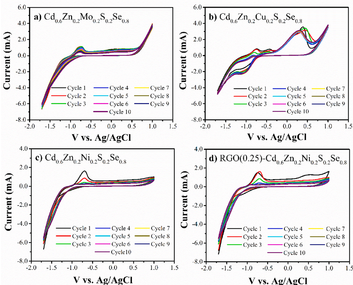
Fig. 2. rCv profiles of a) \text{Cd}_{0.6}\text{Zn}_{0.2}\text{Mo}_{0.2}\text{S}_{0.2}\text{Se}_{0.8} , b) \text{Cd}_{0.6}\text{Zn}_{0.2}\text{Cu}_{0.2}\text{S}_{0.2}\text{Se}_{0.8} , c) \text{Cd}_{0.6}\text{Zn}_{0.2}\text{Ni}_{0.2}\text{S}_{0.2}\text{Se}_{0.8} , d) \text{RGO}(0.25)\text{-Cd}_{0.6}\text{Zn}_{0.2}\text{Ni}_{0.2}\text{S}_{0.2}\text{Se}_{0.8} composite thin films.
