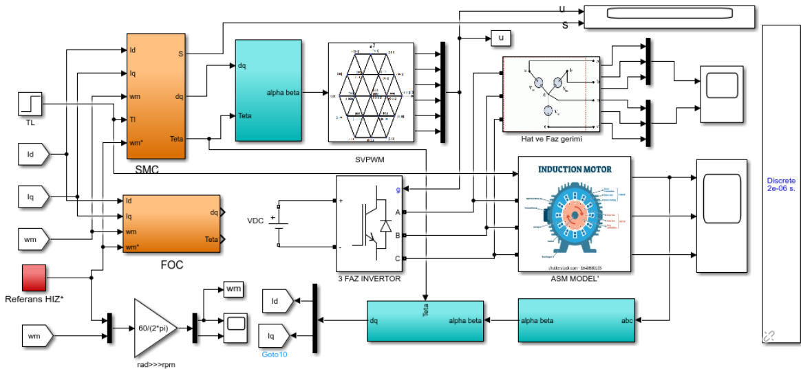
Fig. 2. Simulink model of IM controlled by SMC and FOC.
