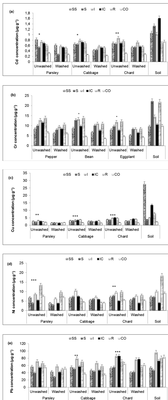
Fig. 2. Mean, Cd (a), Cr (b) Cu (c) Ni (d), Pb (e), and Zn (f) concentrations ( \mu\text{g/g dw} ) in washed, unwashed leaves and soil with Standart Error. Bars, SS: Stream side, S: Suburban, I: Industrial, IC: Inner City, R: Roadside, CO: Control area. Significances of differences between washed and unwashed plants from t-test, are indicated above the columns (* p < 0.05 , ** p < 0.01 , *** p < 0.001 significant).
