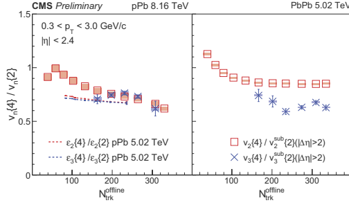
Fig. 2. The ratios of four- and two-particle harmonics ( v_2\{4\}/v_2\{2\} and v_3\{4\}/v_3\{2\} ) are shown for pPb \sqrt{s_{NN}} = 8.16 TeV (left) and PbPb at 5.02 TeV (right) as a function of N_{trk}^{offline} . Error bars and shaded boxes denote statistical and systematic uncertainties, respectively. The dashed curves show a hydrodynamics motivated initial-state fluctuation calculation for pPb collisions at 5.02 TeV [16].
