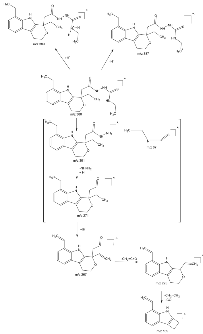
SCHEME 3. MS fragmentation patterns of compound 3b
