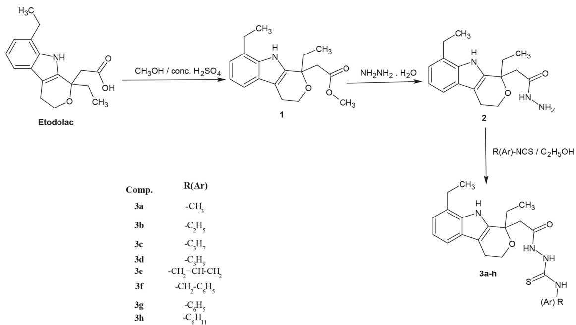
SCHEME 1. Synthetic route of compounds 3a-h.
