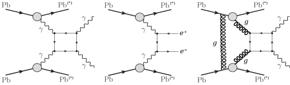
Fig. 1. Diagrams of light-by-light scattering ( \gamma\gamma \rightarrow \gamma\gamma , left), QED dielectron ( \gamma\gamma \rightarrow e^+e^- , center), and central exclusive diphoton ( gg \rightarrow \gamma\gamma , right) production in ultraperipheral PbPb collisions (with potential electromagnetic excitation (^*) of the outgoing Pb ions).
