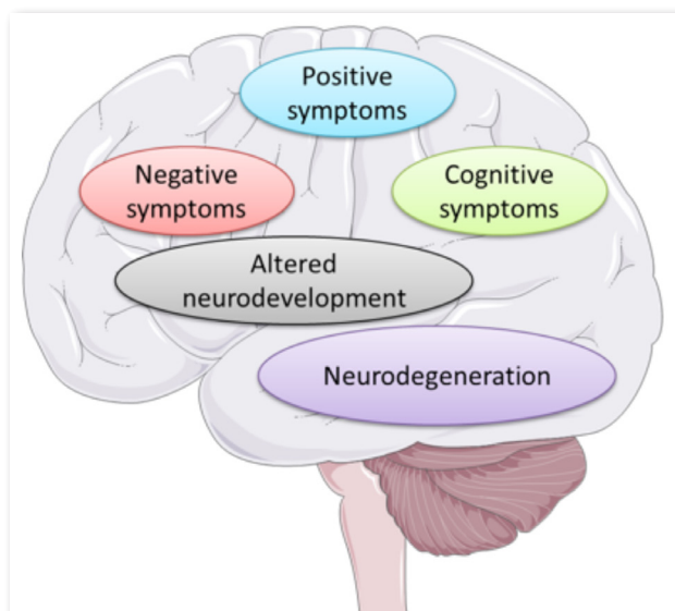
Figure 1: An Overview to Symptoms and Etiology of Schizophrenia. Schizophrenia is a complex and deteriorated disorder that consists of positive, negative, and cognitive symptoms. Positive symptoms include hallucinations and delusions; the negative symptoms include lack of certain abilities seen in normal people such as lack of motivation, cognitive abilities and motivation. For etiology, it is thought that the effect of altered neurodevelopment is dominant in early life while neurodegeneration is responsible in the later ages for schizophrenia.
