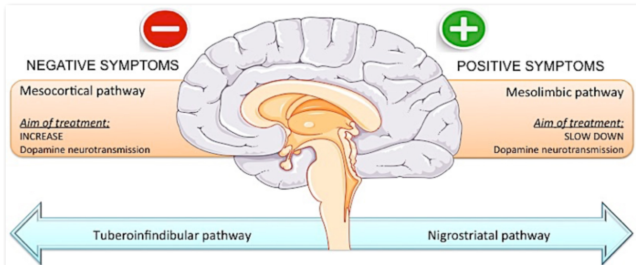
Figure 2: Dopaminergic Hypothesis of Schizophrenia. While hyperactivation of the dopaminergic mesolimbic pathway induces positive symptoms of schizophrenia via increased D2 receptor stimulation in the limbic areas, hypo activation of dopaminergic mesocortical pathway causes negative and cognitive symptoms with decreased D1 receptor activation in the cortical areas. Ideal treatment regimen should decrease the activation of mesolimbic pathway while it should increase the stimulation of cortical areas. Also changing in other pathways' activity (tuberoinfundibular and nigrostriatal pathways) are responsible for side effect of current antipsychotics.
