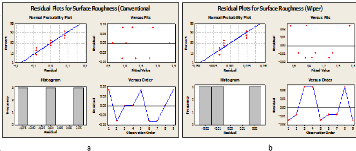
Figure 6. The ANOVA analysis for rate of graphic and feed rate on surface roughness conventional and (b) wiper insert
