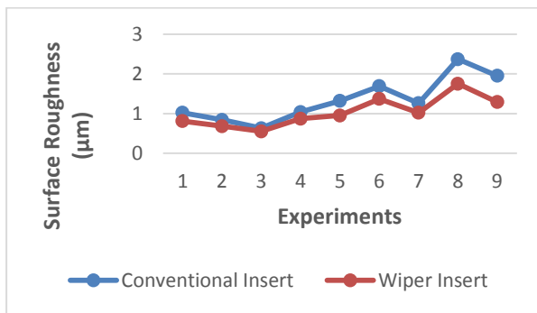
Figure 3. The surface roughness results
