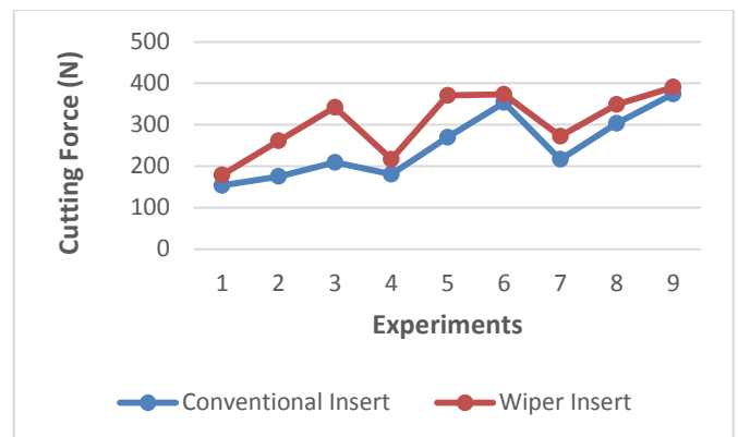
Figure 5. The cutting force results
