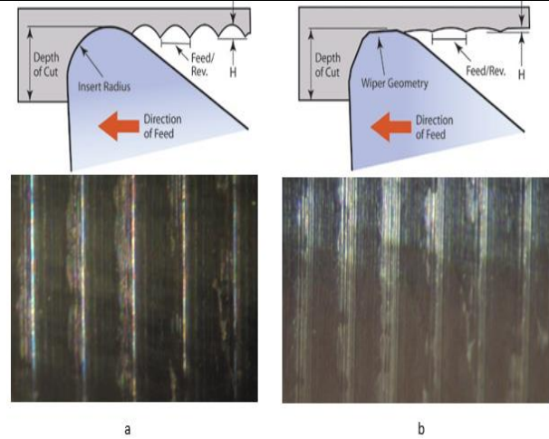
Figure 4. The surface roughness results for (a) conventional and (b) wiper insert
