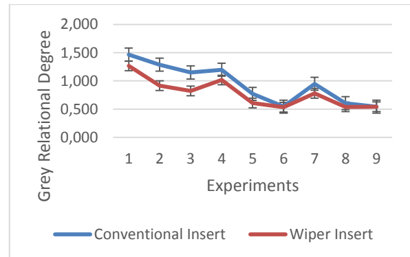
Figure 2. Grey Relational Degrees for each experiments
