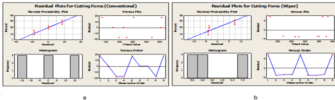
Figure 7. The ANOVA analysis for rate of graphic and feed rate on cutting force conventional and (b) wiper insert
