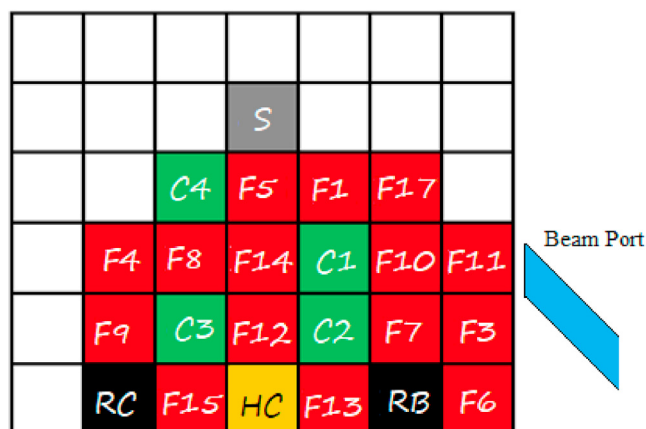
Fig. 2. Current core configuration of MSTR and beam port location (numbers with F represent fuel elements).
