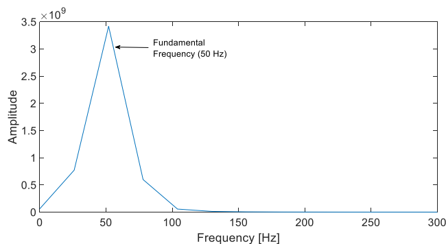
FIGURE 11. Frequency-Power Analysis for Before Ferroresonance
