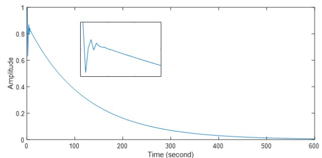
FIGURE 8. Unit Impulse Response of Ferroresonance Phenomena
