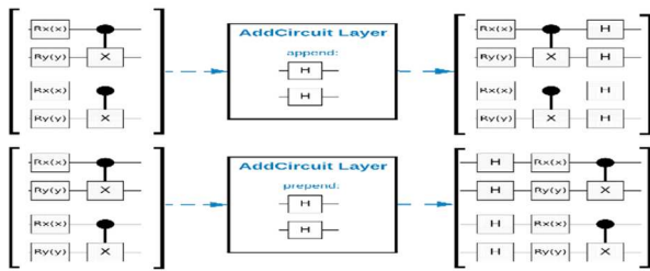
Fig. 5 QCNNs architecture [23]
