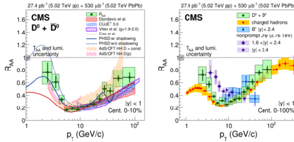
Fig. 2. The left plot shows the D^0 -meson R_{AA} vs p_T in PbPb collisions with centrality of 0 – 10% and the comparison with various theoretical models [8]. The right plot shows the R_{AA} of D^0 mesons, charged hadrons, B^\pm mesons, and non-prompt J/\psi mesons with centrality of 0 – 100% [8].
