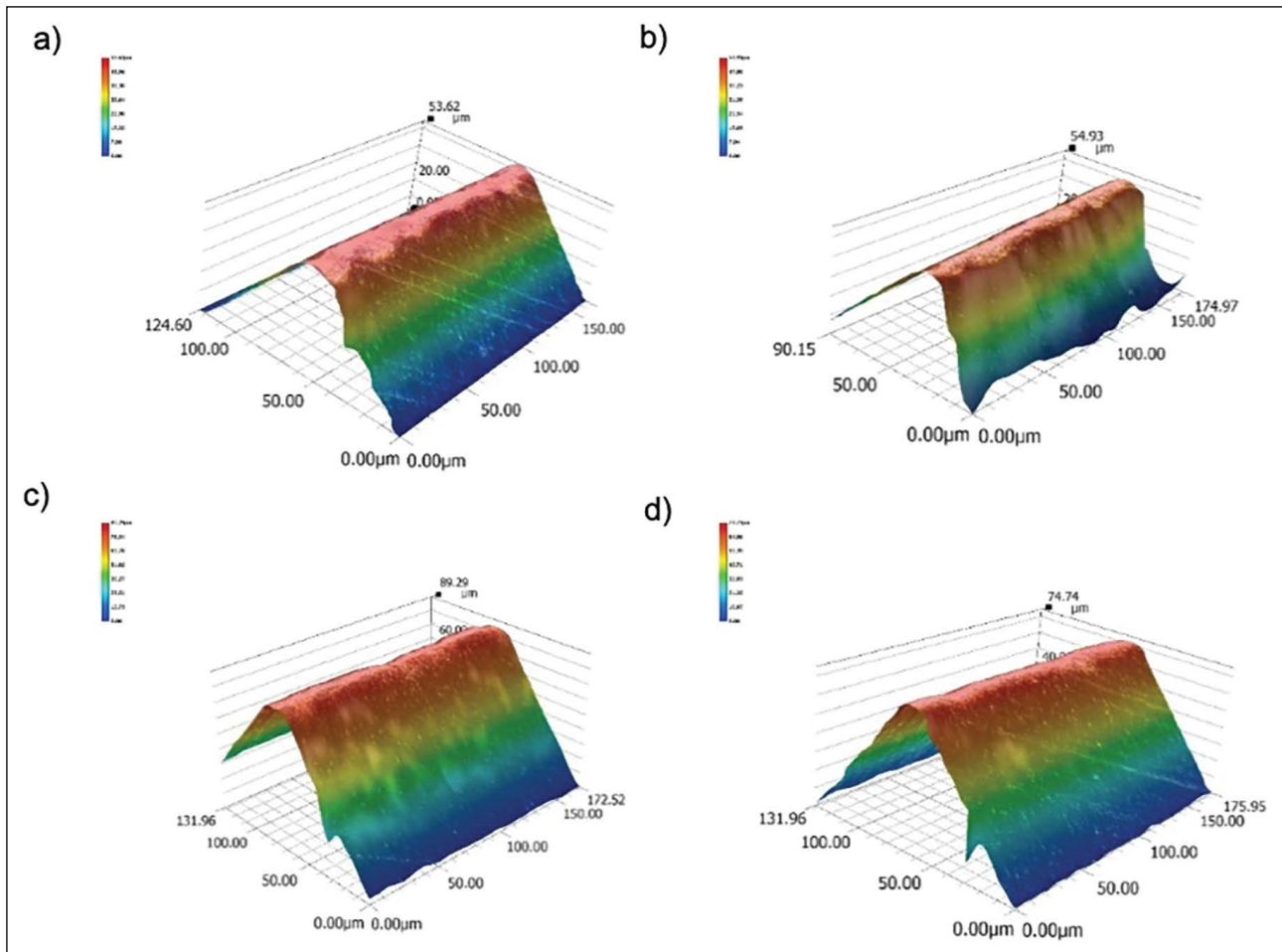
Figure 4. Images of the cutting-edge radius of the tool having 5° of radial rake cutting tool after drag finishing operation; (a) 4 min. (b) 8 min. (c) 20 min. (d) 40 min.
