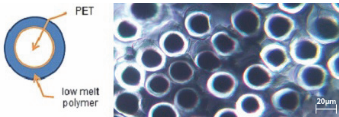
Figure2 -Cross Section of Sheath-Core (50/50) Low Melting Staple PET Polyester Binder Fibre
