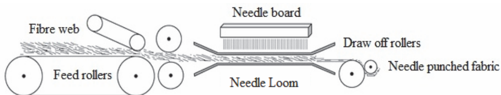
Figure 4. Schematic of the Pre-Needling Machine [27]
