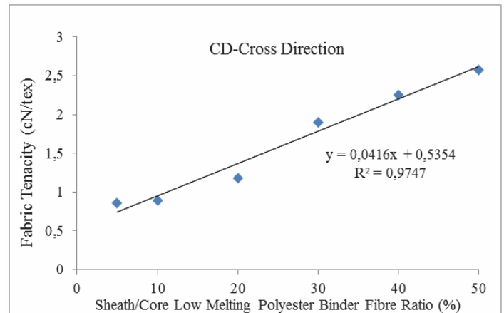
Figure 10. Correlation between sheath/core low melting polyester binder fibre ratio and fabric tenacity of nonwoven fabric in cross direction
