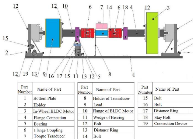
Figure 8. Structure of test setup
