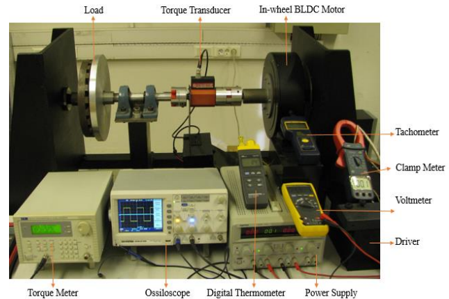
Figure 9. Test setup
