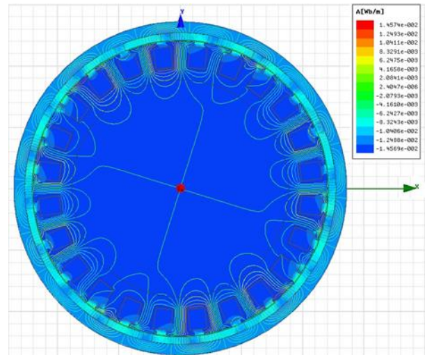
Figure 6. Flux lines of prototyped 24/20 motor
