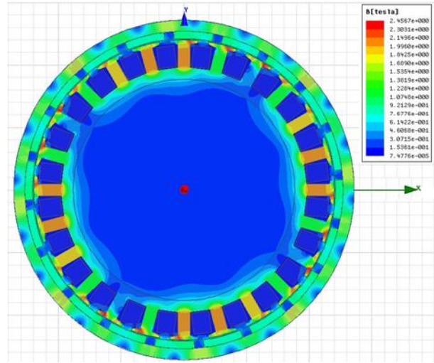
Figure 5. Two dimensional flux density distribution of prototyped 24/20 motor
