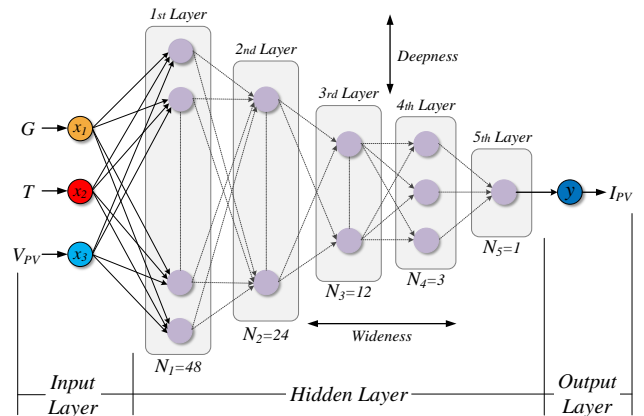
FIGURE 5. Structure of the designed DNN. Weights and bias terms are not shown in the figure to get simplicity. Inputs and outputs are highlighted with different colors, whereas the hidden layer with grey. Adjustment of getting wider structure occurs with adding more hidden layer, while deeper structure requires adding more neuron in the hidden layers.
