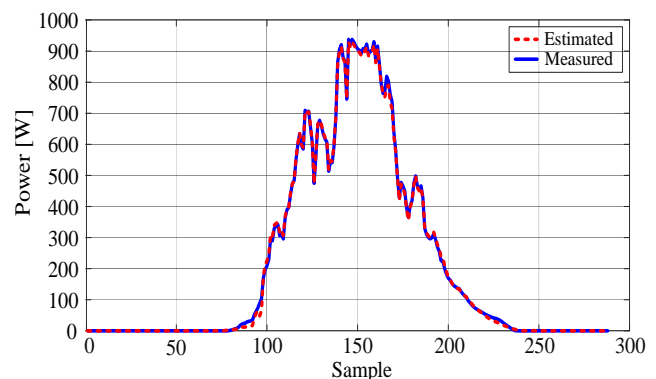
FIGURE 12. Estimated- \hat{P}_{PV} and measured- P_{PV} powers regarding generated power in PV array.
