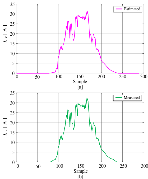
FIGURE 10. [a] Estimated and [b] measured currents for PV converter operation.
