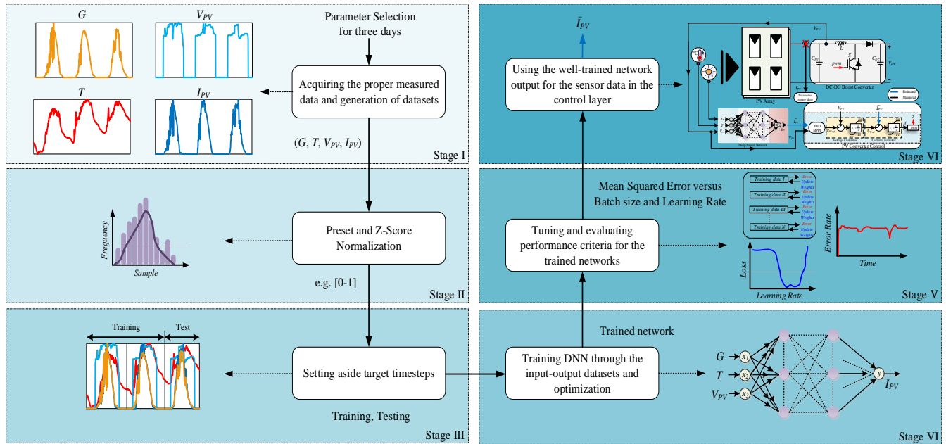
FIGURE 6. Application stages of operation of PV-Battery-based DC nanogrid with deep supervised learning.
