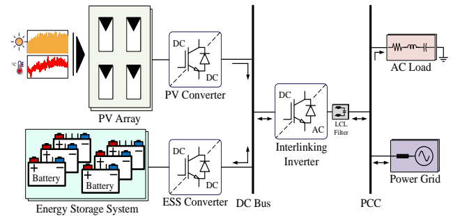
FIGURE 1. Overview of proposed PV-Battery based DC nanogrid.
