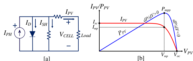
FIGURE 2. [a] Conventional equivalent circuit of PV panel (single diode model) and [b] characteristic curves.
