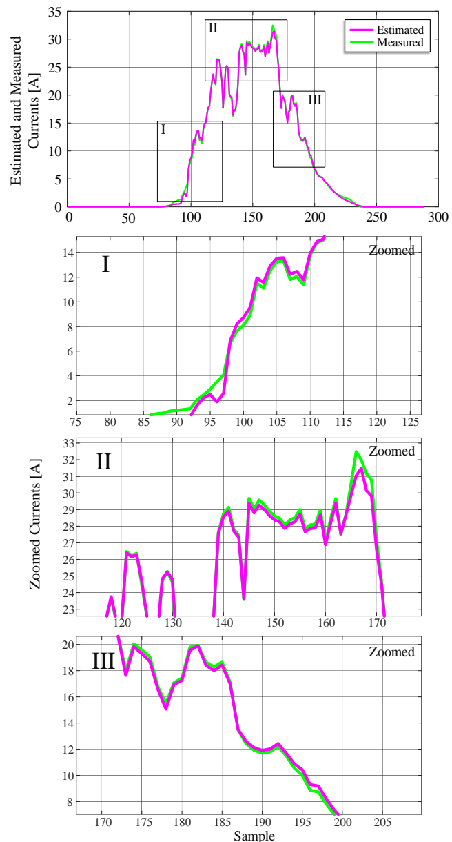
FIGURE 11. Estimated- \hat{I}_{PV} and measured- I_{PV} current values.
