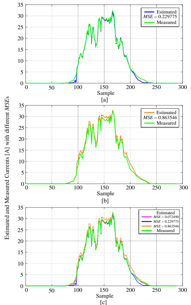
FIGURE 14. Comparison of estimated currents with the measured one. The green line expresses the measured one, while the others are all estimated ones.
