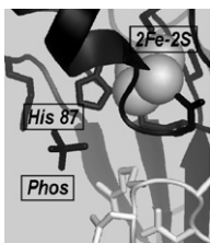
Figure. Part of the crystal structure of mltHET showing the 2Fe-2S cluster (spheres), a cartoon representation of the backbone (black is one dimer and white a symmetry related dimer) and specific amino acids (as labeled) that interact with the bound phosphate anion (black tetrahedron).
