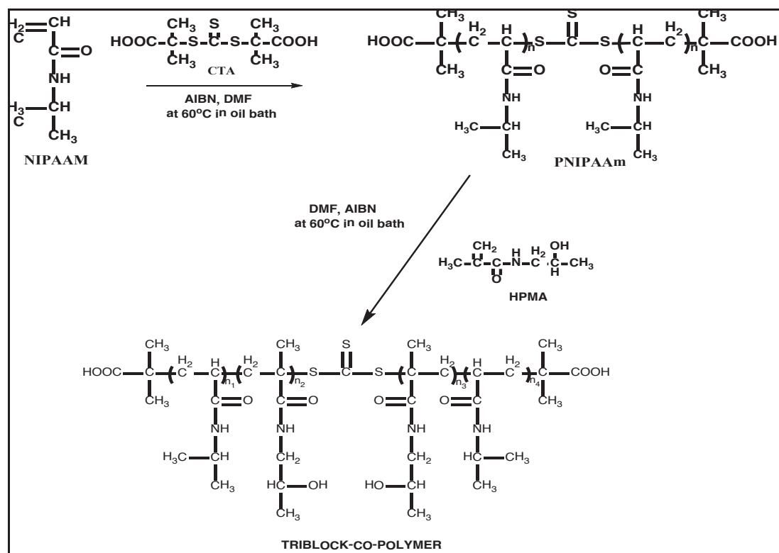
Figure 2. Synthesis of Triblock-co-polymers
