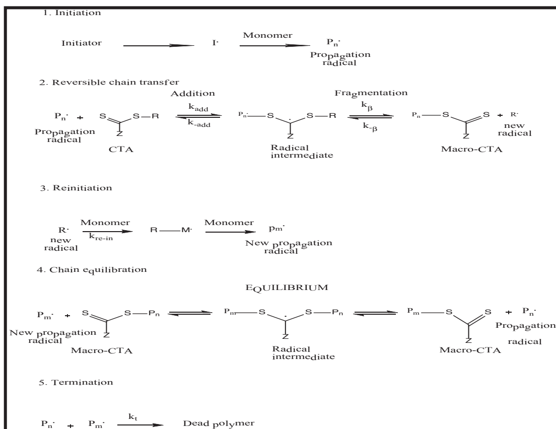
Figure 1. Reversible addition-fragmentation chain transfer (RAFT) polymerization [16-18].
