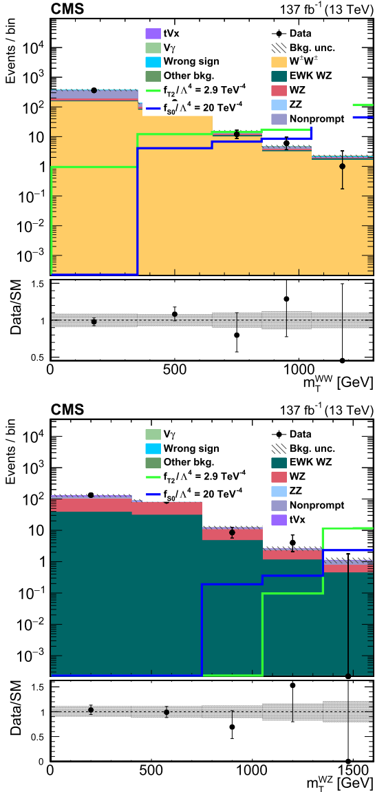
Fig. 6. Distributions of m_T(WW) (upper) in the W^+W^+ SR and m_T(WZ) (lower) in the WZ SR. The gray bands include uncertainties from the predicted yields. The SM predicted yields are shown with their best fit normalizations from the corresponding fits. The contribution of the QCD W^+W^+ process is included together with the EW W^+W^+ process. The overflow is included in the last bin. The bottom panel in each figure shows the ratio of the number of events observed in data to the total SM prediction. The solid lines show the signal predictions for two illustrative aQGC parameters.
