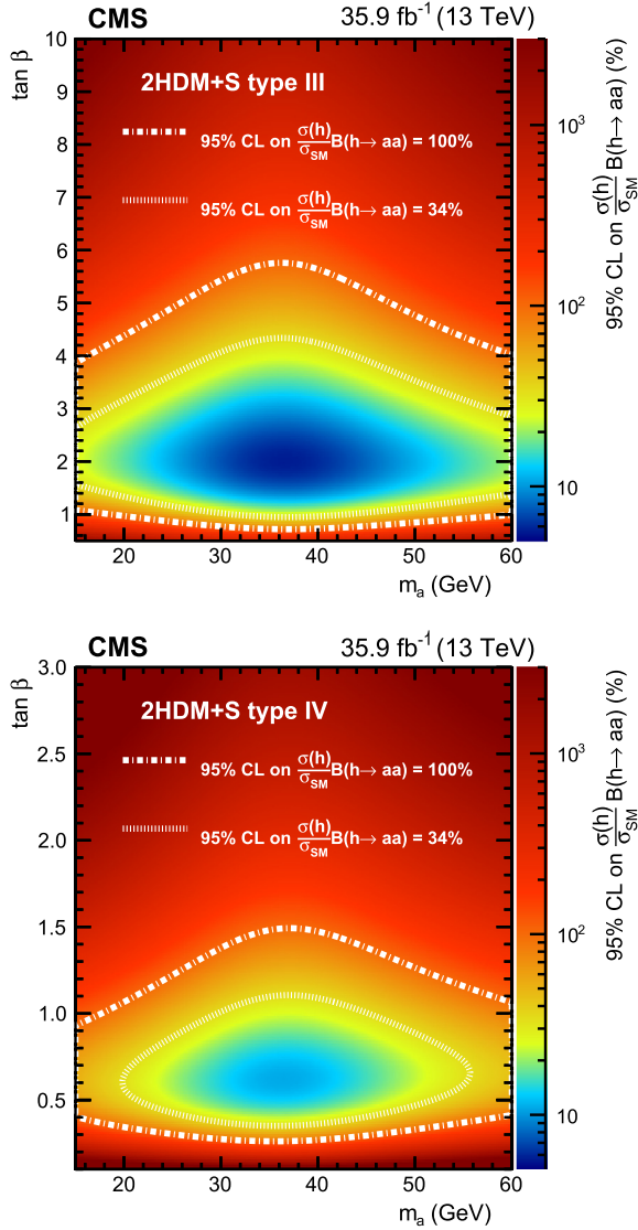
Fig. 8. Observed 95% CL limits on (\sigma(h)/\sigma_{\text{SM}})\mathcal{B}(h \rightarrow aa) in 2HDM + S of type III (top), and type IV (bottom). The contours corresponding to a 95% CL exclusion of (\sigma(h)/\sigma_{\text{SM}})\mathcal{B}(h \rightarrow aa) = 1.00 and 0.34 are drawn with dashed lines. The number 34% corresponds to the limit on the branching fraction of the Higgs boson to beyond-the-SM particles at the 95% CL obtained with data collected at center-of-mass energies of 7 and 8 TeV by the ATLAS and CMS experiments [10].
