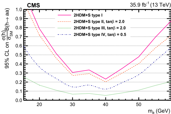
Fig. 9. Observed 95% CL limits on (\sigma(h)/\sigma_{\text{SM}})\mathcal{B}(h \rightarrow aa) for various 2HDM + S types. The limit in type I 2HDM + S does not depend on \tan\beta .
