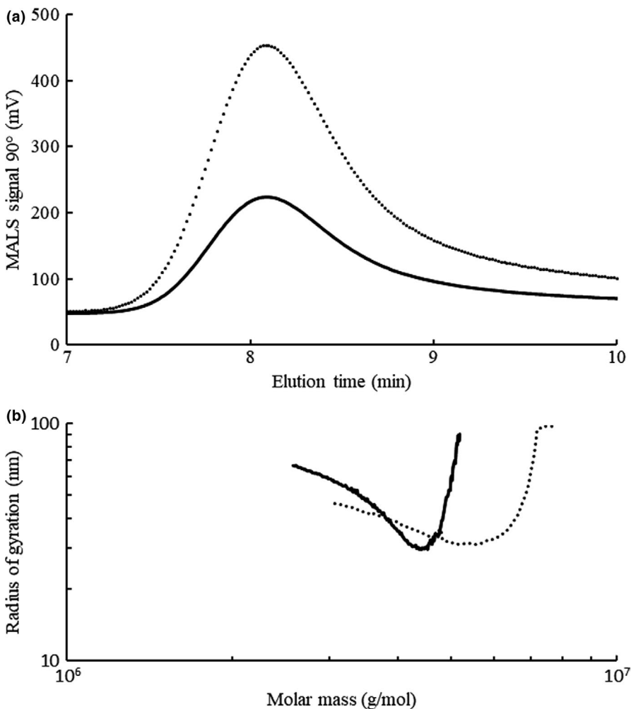
FIGURE 3 SEC-MALS Elution profile (a) and conformation plot (b) for levan EH (.....) and levan HS (—)
