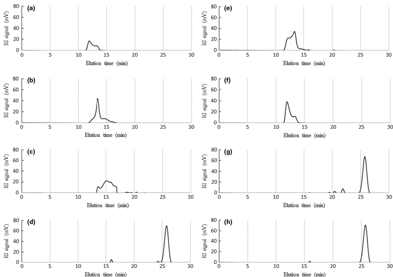
FIGURE 5 Elution profiles from gel permeation chromatography of the hydrolysis products of levan EH at (a) 120°C, (b) 140°C, (c) 160°C, and (d) 180°C, and levan HS at (e) 120°C, (f) 140°C, (g) 160°C, and (h) 180°C
