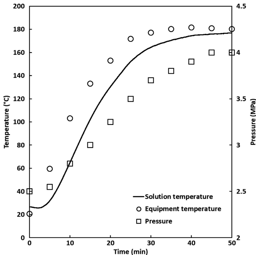
FIGURE 1 Typical behavior of the equipment temperature, solution temperature, and pressure during the hydrolysis of levan using compressed hot water fluids
