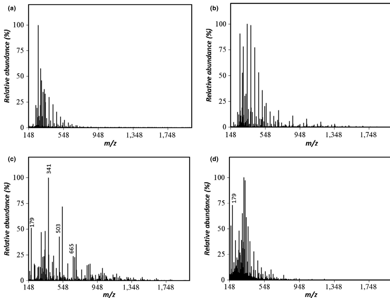
FIGURE 6 ESI-MS spectra (negative-ion mode) of the levan HS hydrolysate prepared by the compressed hot water process at (a) 120°C, (b) 140°C (c) 160°C, and (d) 180°C
