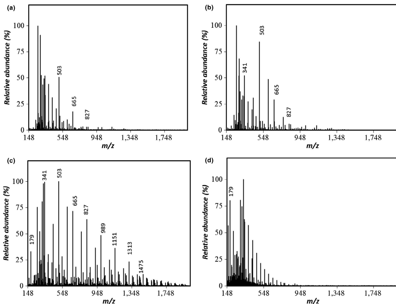
FIGURE 7 ESI-MS spectra (negative-ion mode) of the levan EH hydrolysates prepared by the compressed hot water process at (a) 120°C, (b) 140°C (c) 160°C, and (d) 180°C
