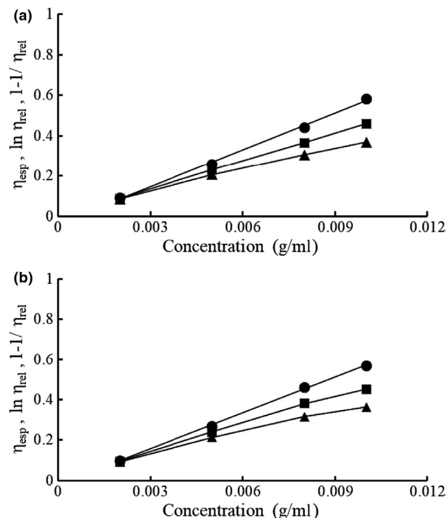
FIGURE 4 Tangletpaibul-Rao (●), Higiro 1 (■), and Higiro 2 (▲) plots of levan HS (a) and levan EH (b) at 25°C
