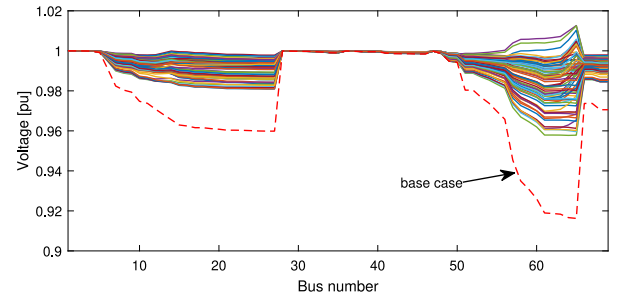
Fig. 12. Voltage magnitude profiles in 69-bus test system for the CPS and the base case (6 p.m. of the summer day).
