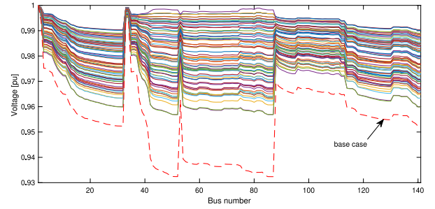
Fig. 16. Voltage magnitude profiles in 141-bus test system for the CPS and the base case (6 p.m. of a summer day).
