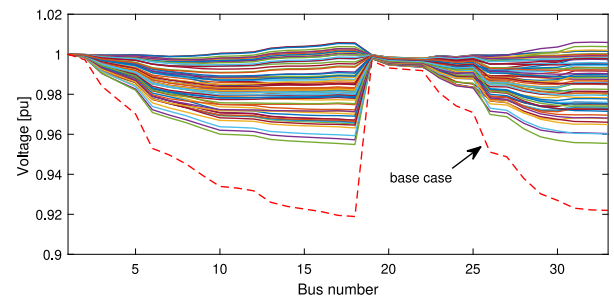
Fig. 8. Voltage magnitude profiles in 33-bus test system for the CPS and the base case (6 p.m. of the summer day).
