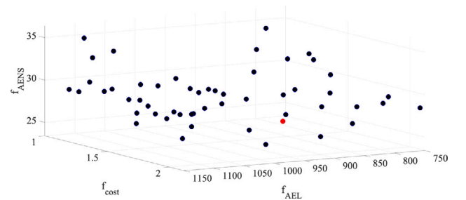
Fig. 13. Pareto optimal solution for Case Study III.
