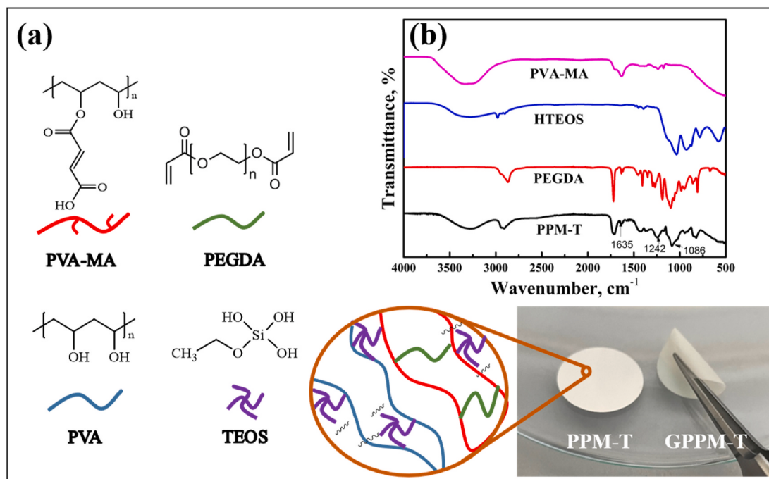
Fig. 3. (a) Composition and photo image (illustration) of the dry PPM-T membrane and GPPM-T gel electrolyte, and (b) FTIR spectra of DCNM.
