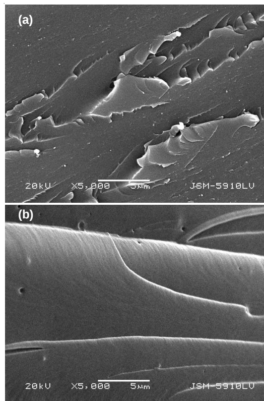
Fig. 10. SEM images of fracturesurfaces of (a) HF-0 (b) HF-7.5 samples
