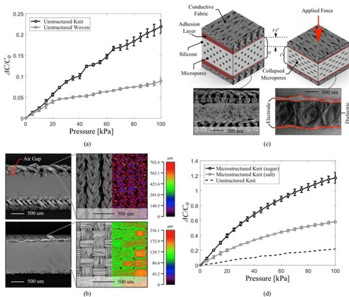
Figure 2. (a) Relative change in sensors' capacitance under pressure for the sensors consists of unstructured dielectric layer with the knit and woven electrodes. (b) SEM images show the surface properties of the knit and woven electrodes as well as air gaps within structure. (c) Working mechanism of the micro-porous sensors, SEM images shows before and after loading. (d) Relative change in sensors' capacitance under pressure for the sensors consists of mpdl (either sugar or salt crystal) with the knit electrodes.
