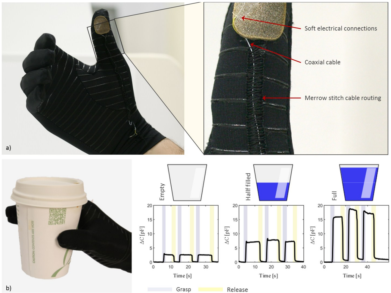
Figure 4. (a) An image shows the sensing glove with its components. (b) Graphics shows the change in capacitance values when the subject grasps the different amount weights.
