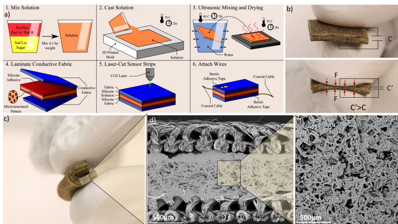
Figure 1. (a) Schematic diagram of the fabrication process of the capacitive based soft pressure sensor. (b) Actual image of the sensor and general working principle under force loading. (c) Actual image of the sensor in which bendability of the sensor is shown. (d) Cross-sectional view of the sensor captured via SEM. (e) SEM image of the mpdl
