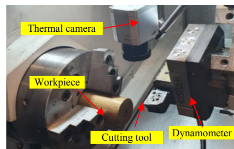
Fig. 2. Experimental setup.
