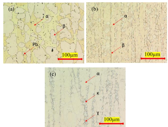
Fig. 1. Microstructure of (a) CW617N; (b) CW511L; (c) CW724R.
