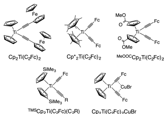
Figure 1. \text{Fe}^{\text{II}}\text{-Ti}^{\text{IV}} complexes discussed in this paper along with abbreviations used. {}^{\text{R}}\text{Cp}_2\text{Ti}(\text{C}_2\text{Fc})_2 is the abbreviation used to refer to the complexes with two ethynylferrocene ligands and any substitution on the Cp ring (top row).
