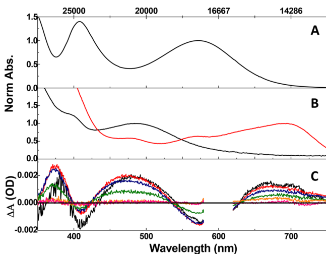
Figure 4. (A) Electronic absorbance spectrum of \text{Cp}_2\text{Ti}(\text{C}_2\text{Fc})_2 . (B) Electronic absorbance of reduced \text{Cp}_2\text{Ti}(\text{C}_2\text{Fc})_2 (black) and oxidized \text{HC}_2\text{Fc} (red). (C) Select transient spectra of \text{Cp}_2\text{Ti}(\text{C}_2\text{Fc})_2 with 600 nm excitation at time delays of 0.32 (black), 1.5 (red), 6.0 (blue), 24 (green), 96 (orange), and 180 ps (pink). The laser line for the pump–probe data has been removed, and a reference zero line has been added for ease of interpretation.
