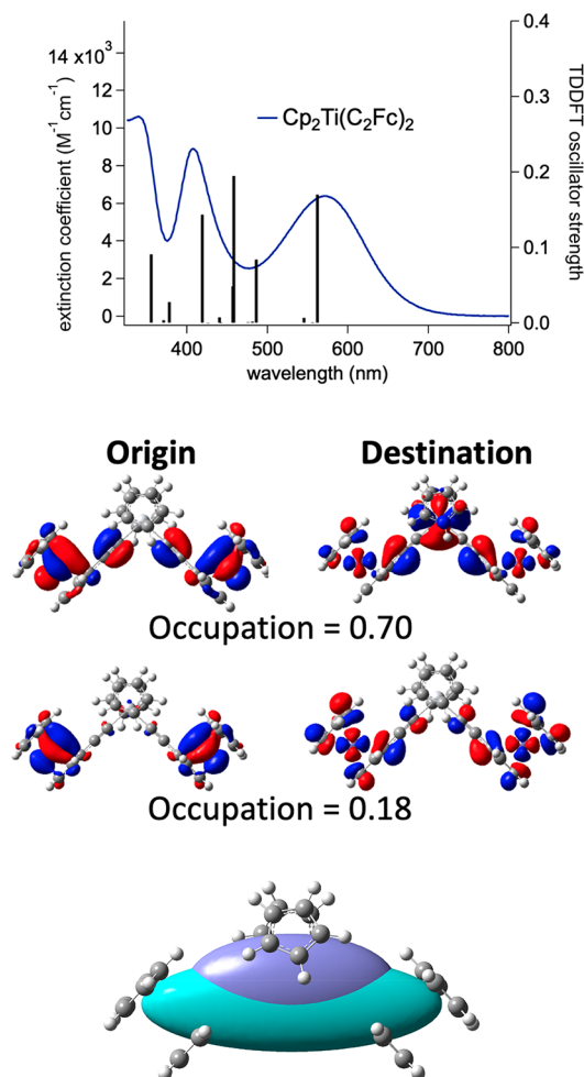
Figure 6. Top: Experimental electronic absorbance spectrum of \text{Cp}_2\text{Ti}(\text{C}_2\text{Fc})_2 along with calculated transitions and oscillator strengths (vertical bars). Note: No shift or offset is applied to the calculated transitions. Middle: Diagrams of the origin and destination NTOs with the highest eigenvalues for the lowest-energy transition. Bottom: Diagram depicting the shape of the barycenters for charge accumulation (violet, closest to Ti) and charge depletion (teal, closest to Fe) as calculated by TDDFT for \text{Cp}_2\text{Ti}(\text{C}_2\text{Fc})_2 . A default isovalue density of 0.0004 is used for all surfaces.
