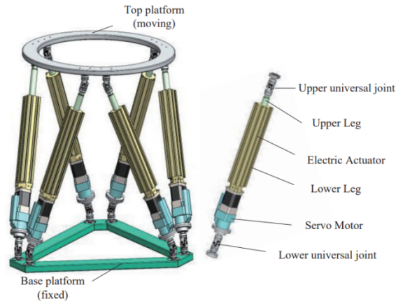
FIGURE 1. Stewart Platform [3].
