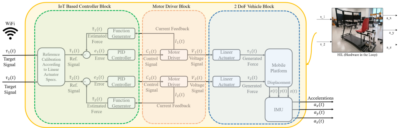
FIGURE 5. Hardware in the Loop (HIL) for 2 DoF Vehicle Simulator.
