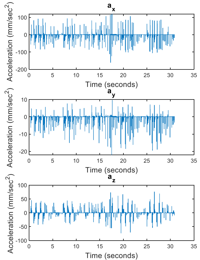
FIGURE 8. HIL Responses for System Identification Inputs.
