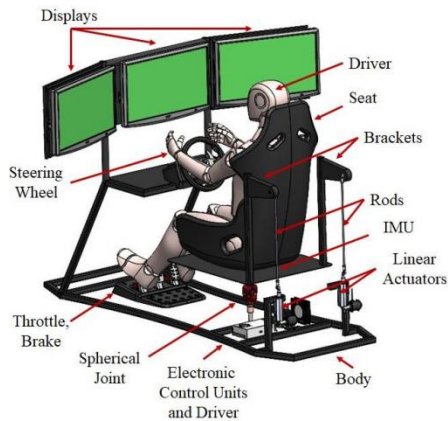
FIGURE 2. 2 DoF Vehicle Simulator Conceptual Design.
