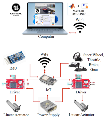
FIGURE 3. Hardware Architecture of 2 DoF Vehicle Simulator.
