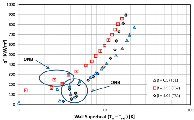
Figure 13. Effect of aspect ratio on boiling curve for G = 800 \text{ kg/(m}^2\text{s)} at z/L = 0.6 .
