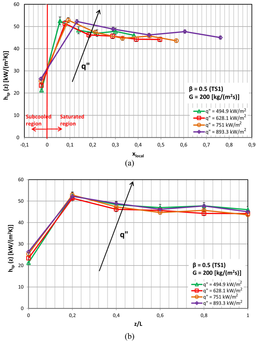
Figure 15. Effect of high heat flux input on the local heat transfer coefficient for the TS1 at 200 \text{ kg}/(\text{m}^2\text{s}) ; (a) versus local vapor quality and (b) versus axial distance.
