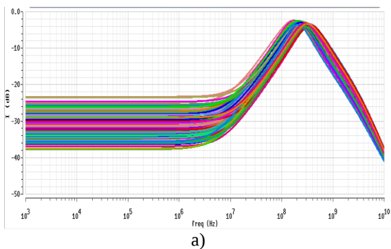
Figure 13. Monte-Carlo simulation of the design 2: a) Frequency response of the BP output, b) Center frequency variation.
