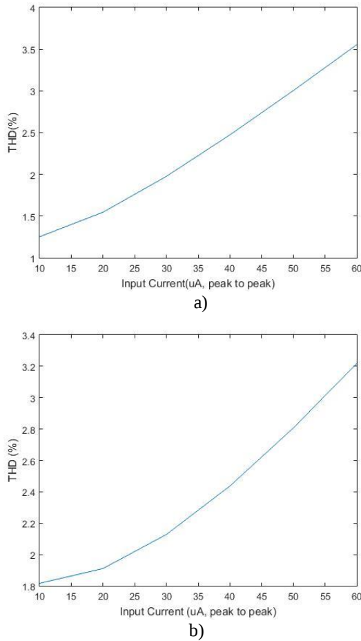
Figure 11. THD result of the exemplary designs: a) Design 1, b) Design 2.
