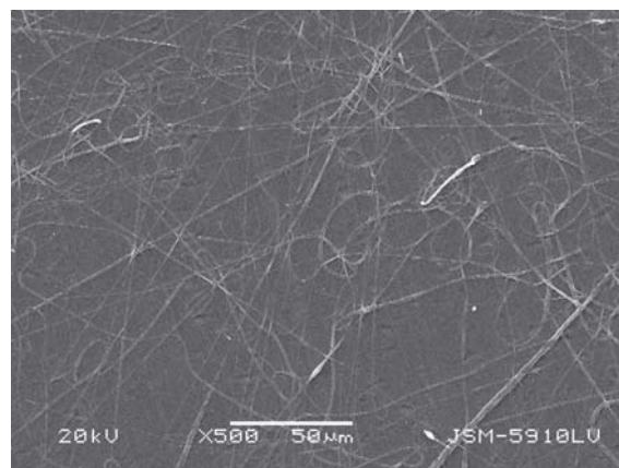
Figure 5. SEM image of SEBS-g-MA+CNW electrospun nanofiber without water inclusion.
