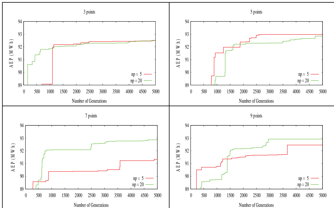
Figure 5 Evolution of AEP obtained using macroevolutionary algorithm with different population sizes.
