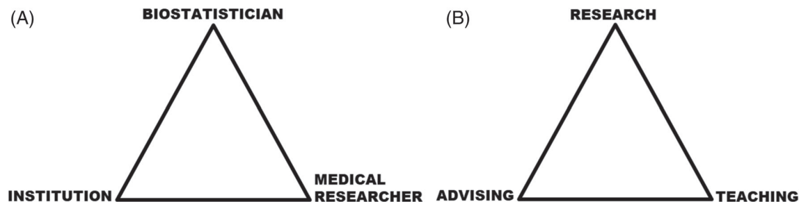
FIGURE 1 The golden triangles of (A) biostatistical advising and (B) the components of a biostatistician's career
